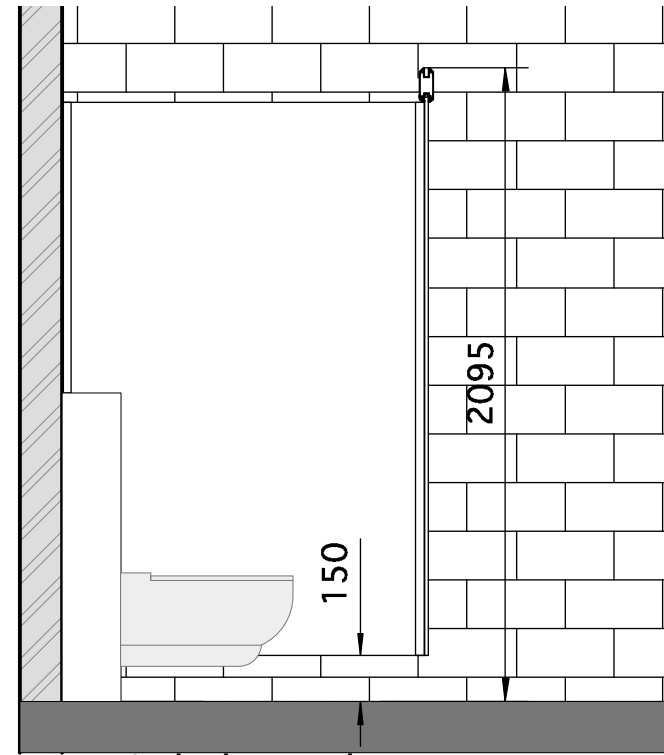
verticale doorsnede coupe verticale vertical view
